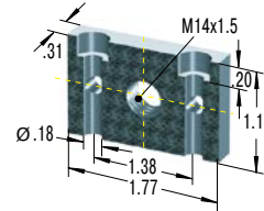
250-0352 Mounting Block
