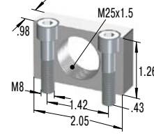
250-0436 Mounting Block
