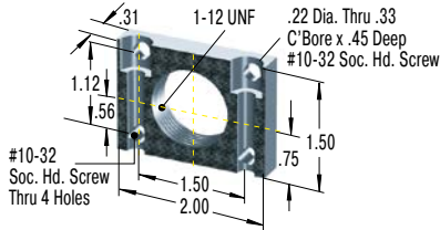
250-0402 Mounting Block
