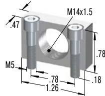
250-0255 Mounting Block
