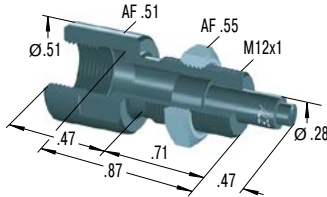
250-0760 Side Load Adaptor
