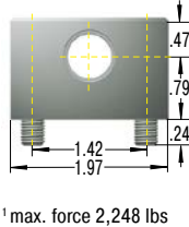
ND14 Mounting Flange
