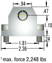
ME14 Bearing Shoe
