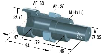
250-0558 Side Load Adaptor
