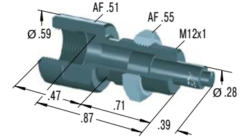
250-0145 Side Load Adaptor
