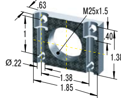
250-0044 Mounting Block
