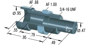
250-0561 Side Load Adaptor
