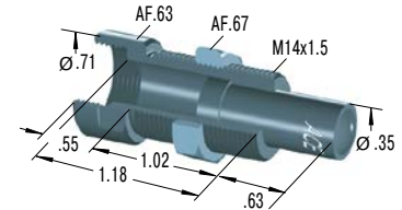
250-0080 Side Load Adaptor
